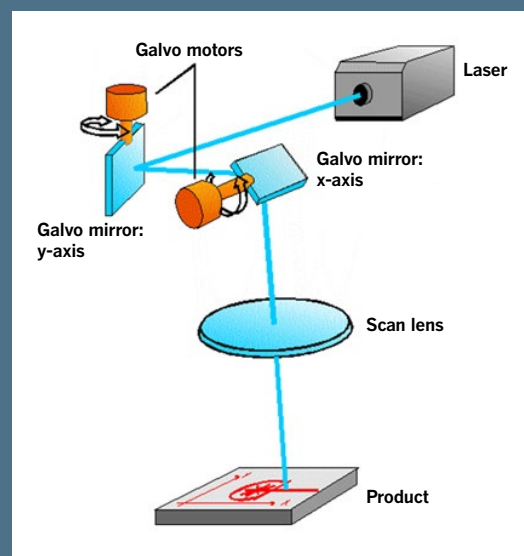
CO 2 laser technology diagram
