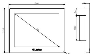
COMMANDER 110S
